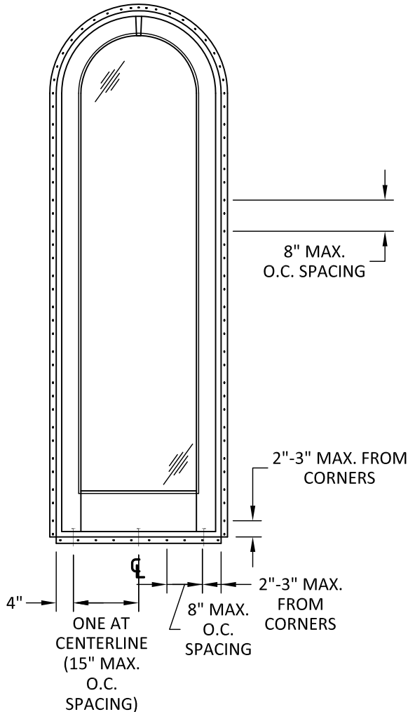
ANCHOR LAYOUT NAIL FIN
