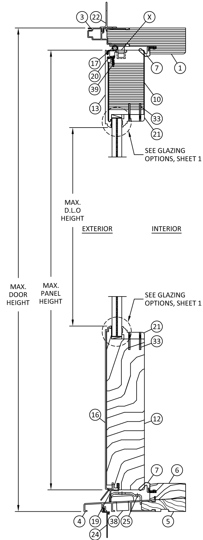
B 8 VERTICAL SECTION NAIL FIN OPERABLE DOOR
