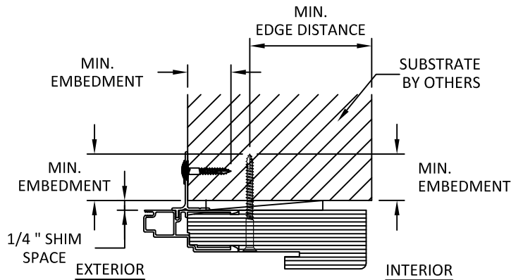
A 12 ANCHOR DETAIL NAIL FIN (HEAD)
