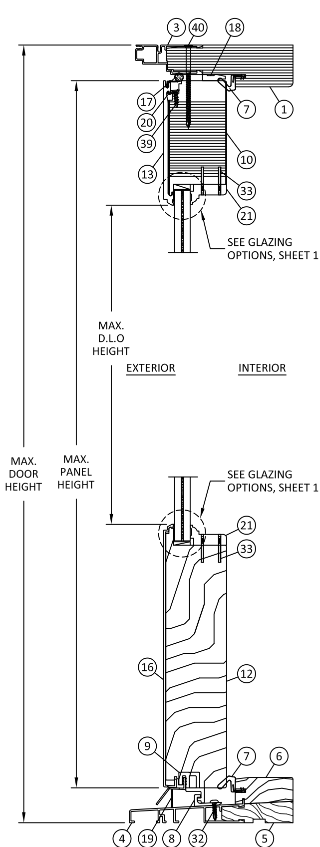
A 7 VERTICAL SECTION THROUGH FRAME FIXED DOOR
