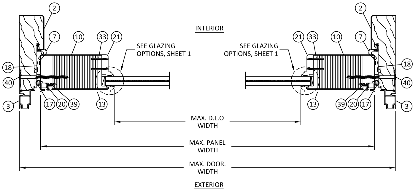
A HORIZONTAL SECTION 9 JAMB OUTSWING
