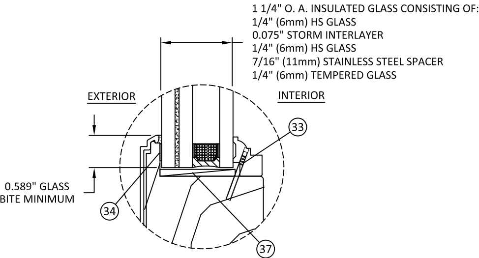
GLAZING DETAIL 2
