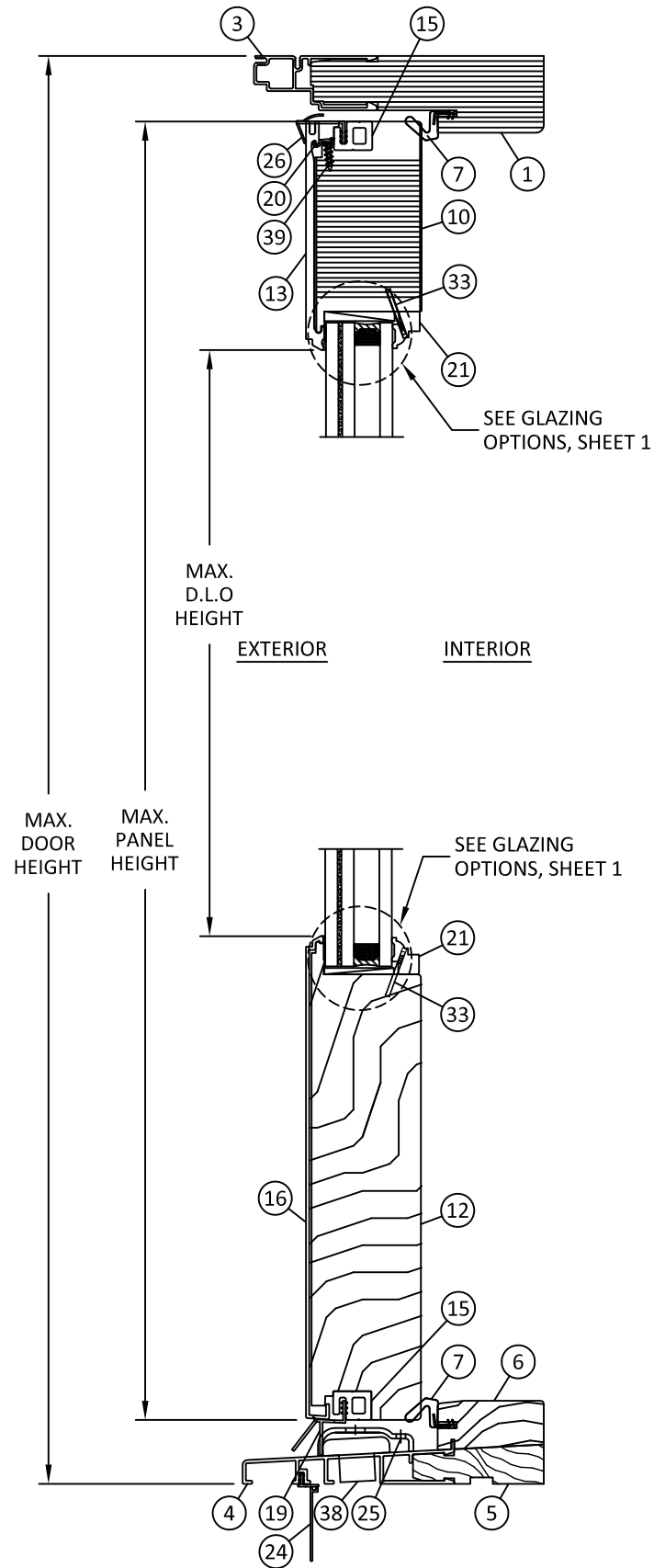
A 8 VERTICAL SECTION THROUGH FRAME OPERABLE DOOR
