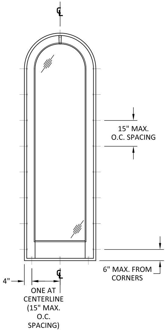
ANCHOR LAYOUT THROUGH FRAME
