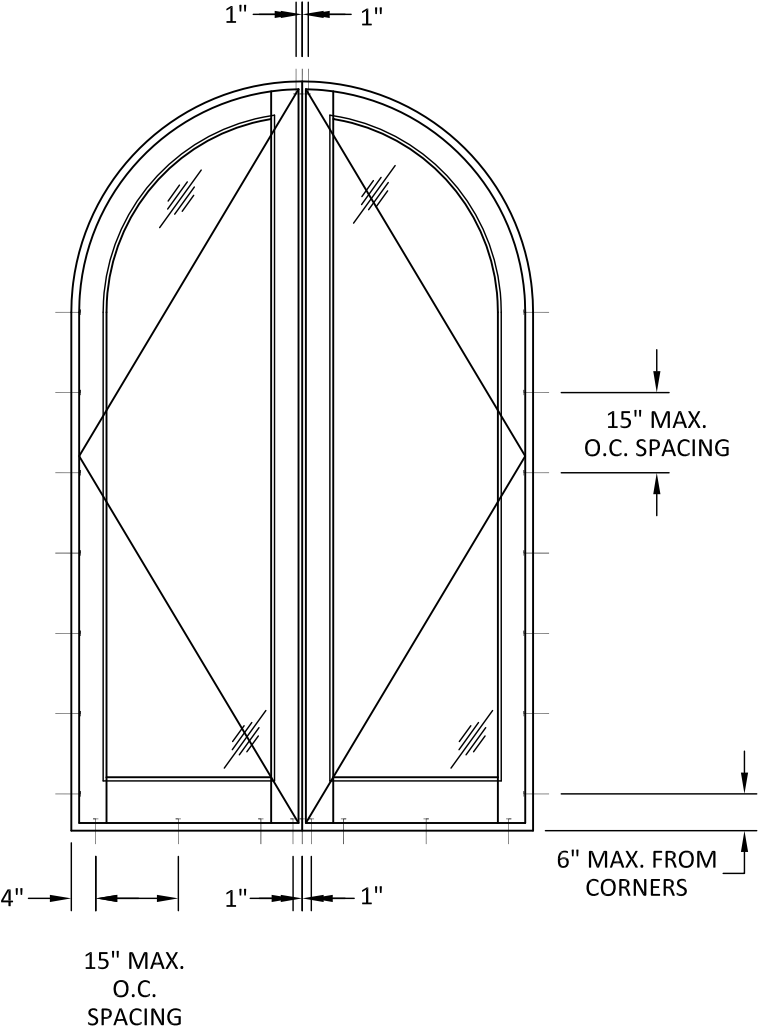
ANCHOR LAYOUT THROUGH FRAME
