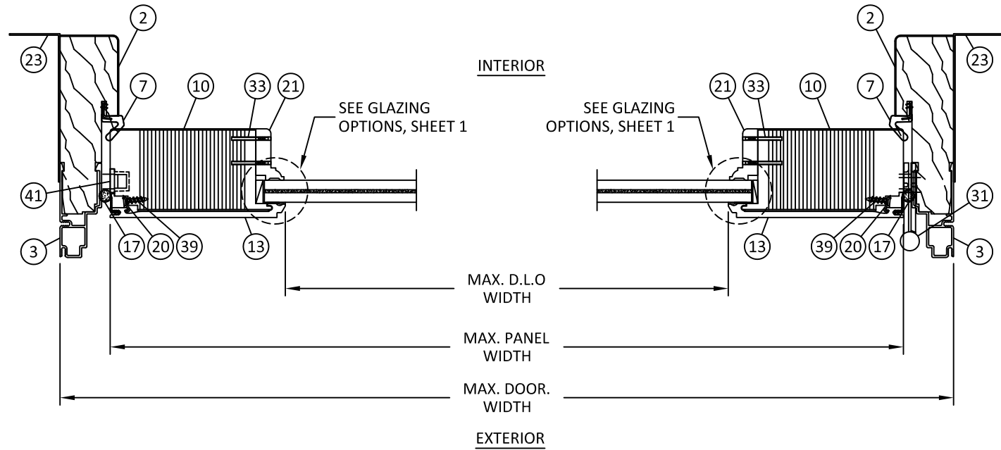
A HORIZONTAL SECTION 10 JAMB OUTSWING
