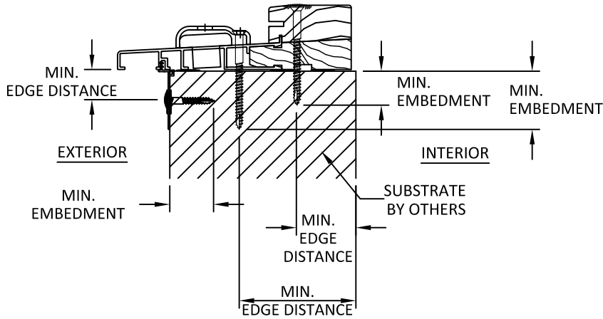
B 12 ANCHOR DETAIL NAIL FIN (OPERABLE SILL)
