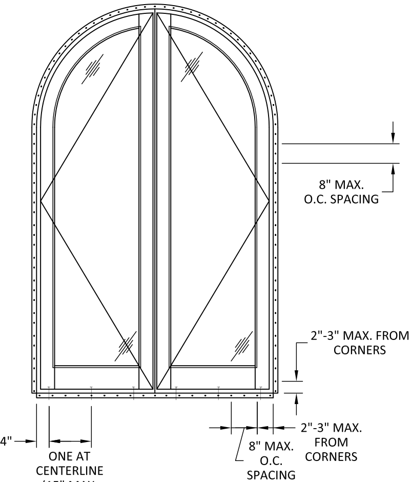
ANCHOR LAYOUT NAIL FIN
