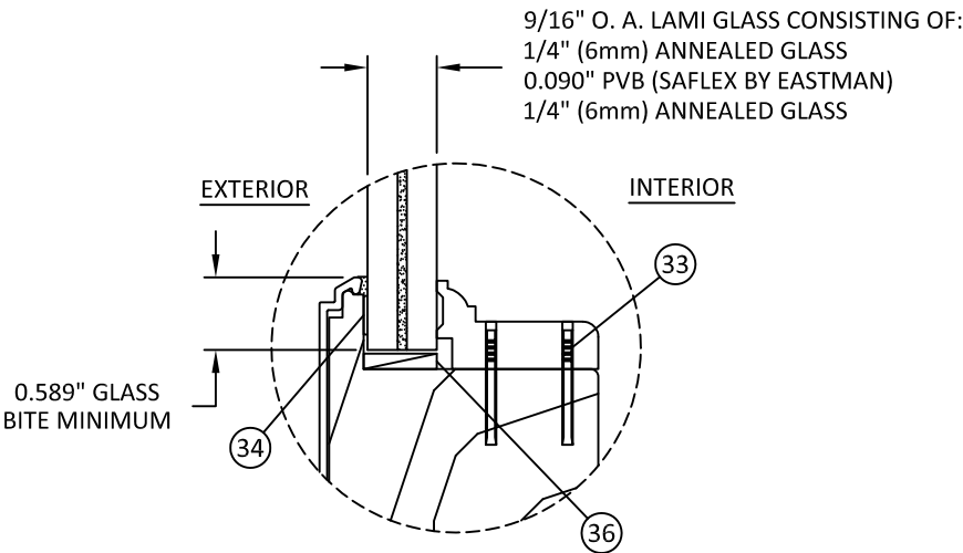
GLAZING DETAIL 1
