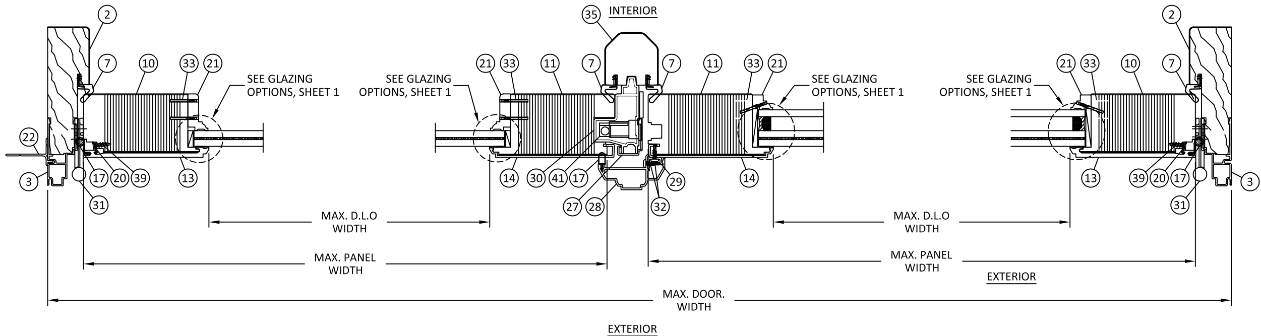
C HORIZONTAL SECTION 10 JAMB OUTSWING
