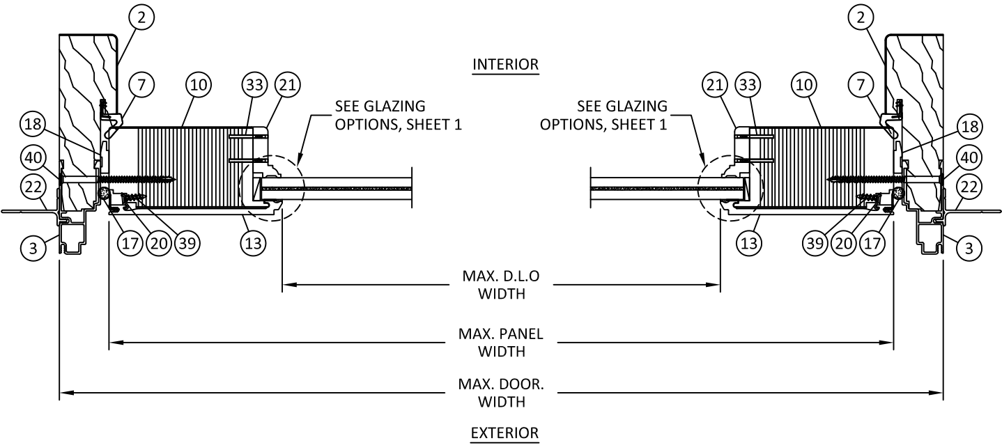
C HORIZONTAL SECTION 9 JAMB OUTSWING
